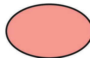
oval
