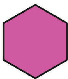
hexagon
